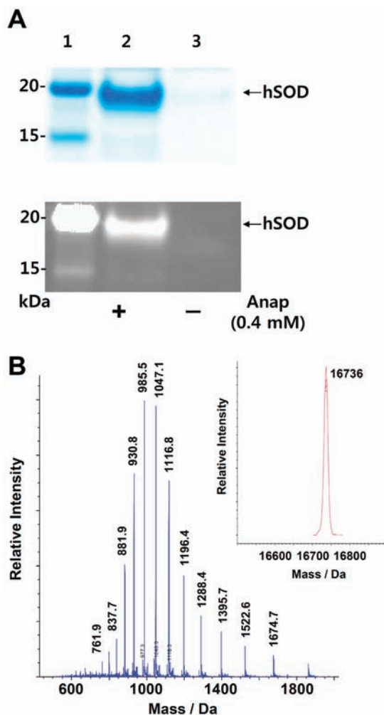
Figure 2. Expression of hSOD with an amber codon at position 33 in the presence of the \text{tRNA}_{\text{CUA}}^{\text{Leu}}/\text{Anap-2C} pair and 0.4 mM Anap. (a) SDS-PAGE analysis by GelCode Blue staining (top) and fluorescence (bottom). Lane 1, protein marker; Lane 2, hSOD expressed in the presence of the \text{tRNA}_{\text{CUA}}^{\text{Leu}}/\text{Anap-2C} pair and 0.4 mM Anap; Lane 3, hSOD expressed in the presence of the \text{tRNA}_{\text{CUA}}^{\text{Leu}}/\text{Anap-2C} pair, but in the absence of Anap. (b) ESI-MS analysis. The inset shows the deconvoluted spectrum: calculated 16 738, observed 16 736.
